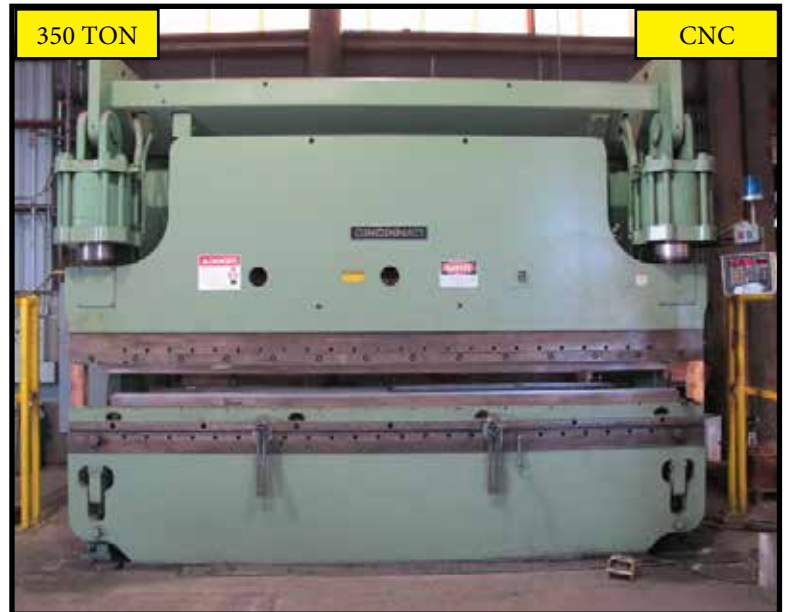
1978 Cincinnati mdl. 350CB X 12 350 Ton x 12' Hydraulic CNC Press Brake s/n 41268 w/ Automec Auto Gauge 1000 CNC Controlled Back Gauging
