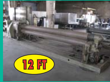
WEBB MODEL 6L, 12FT x 3/16" INITIAL PINCH PLATE ROLLS
